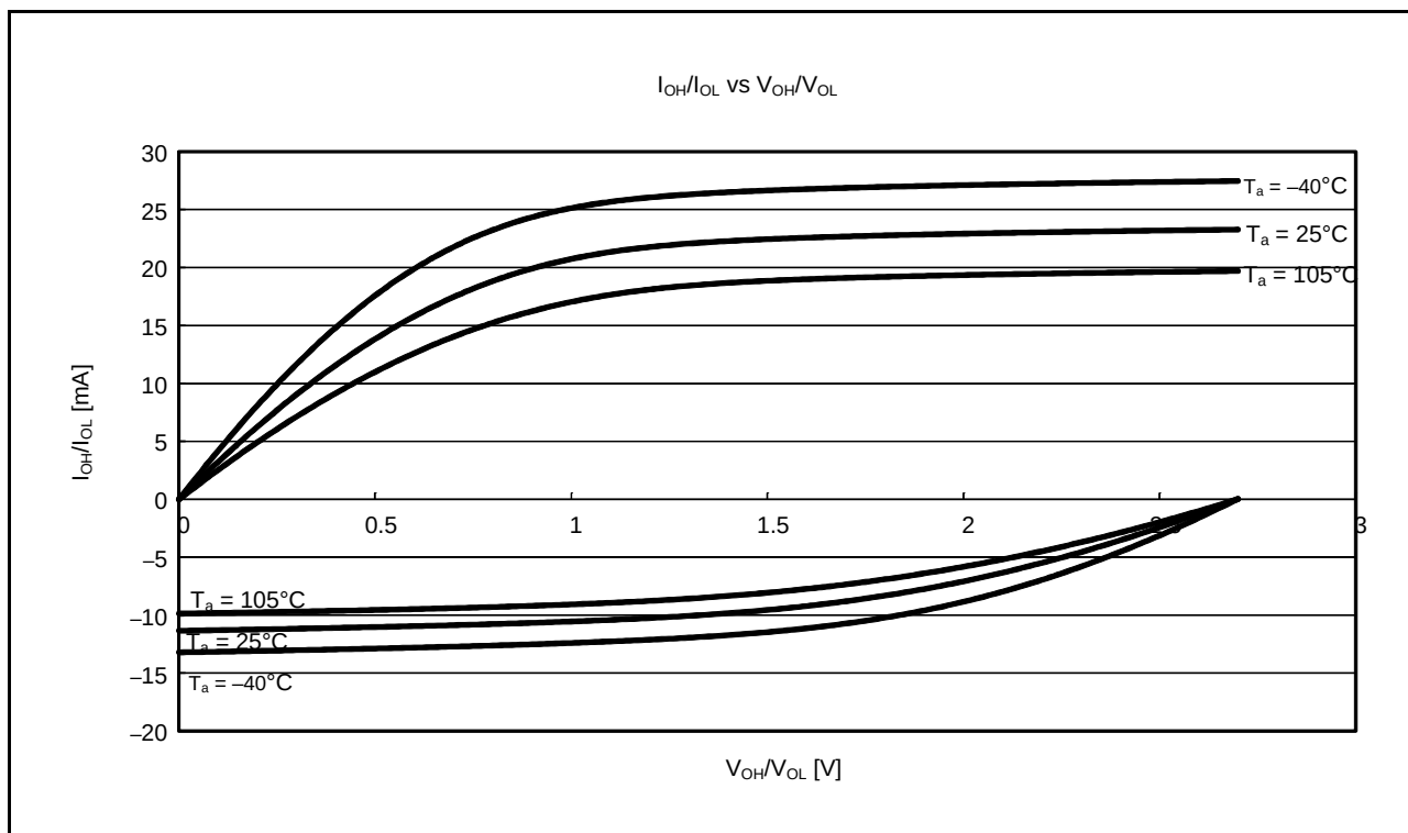
Figure 5.9 V_{OH}/V_{OL} and I_{OH}/I_{OL} Temperature Characteristics of General Ports (Except for the RIIC Output Pin, Ports P40 to P44, P46, Ports PJ6, PJ7) at V_{CC} = 2.7\text{ V} (Reference Data)
