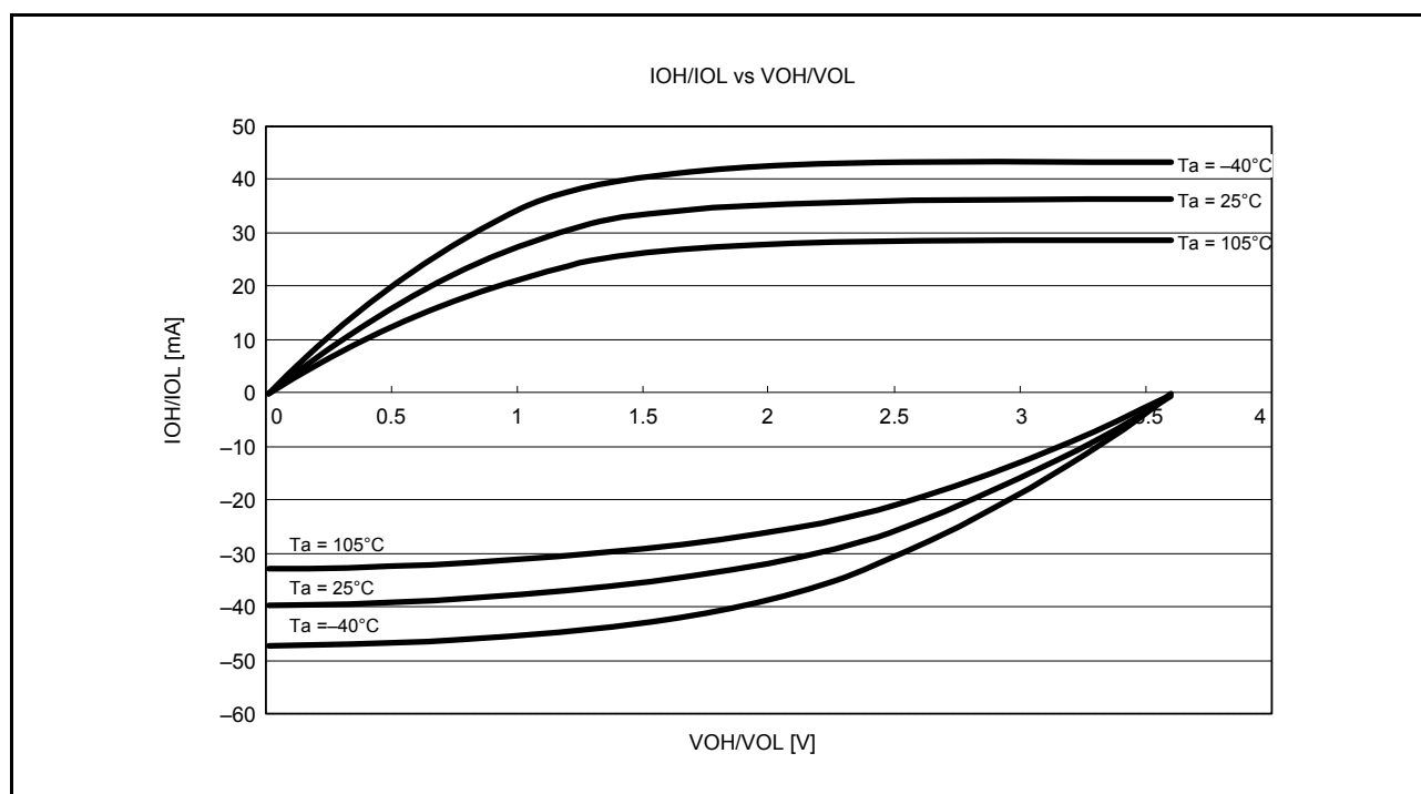
Figure 5.20 V_{OH}/V_{OL} and I_{OH}/I_{OL} Temperature Characteristics at V_{CC} = 3.6\text{ V} when High-Drive Output is Selected (Reference Data)
