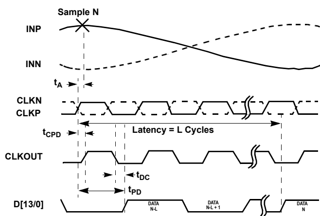
Figure 5. SDR
