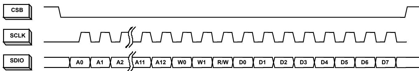
Figure 37. LSB-First Addressing
