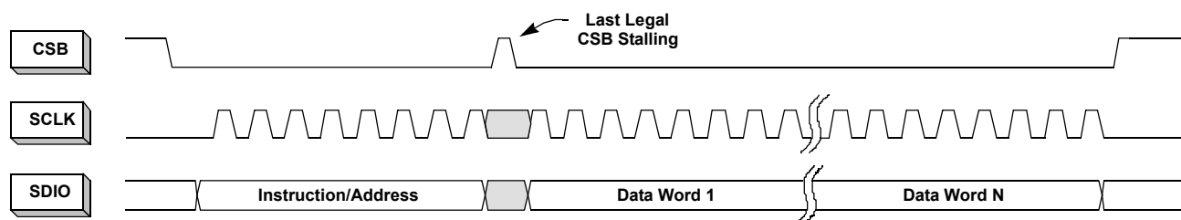
Figure 41. N-Byte Transfer
