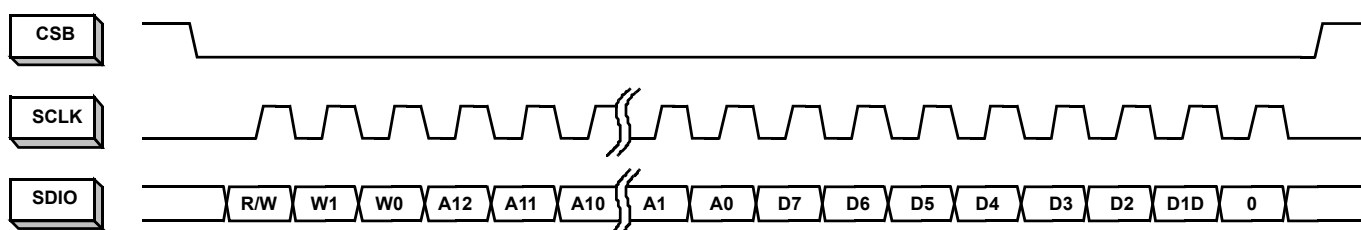
Figure 36. MSB-First Addressing
