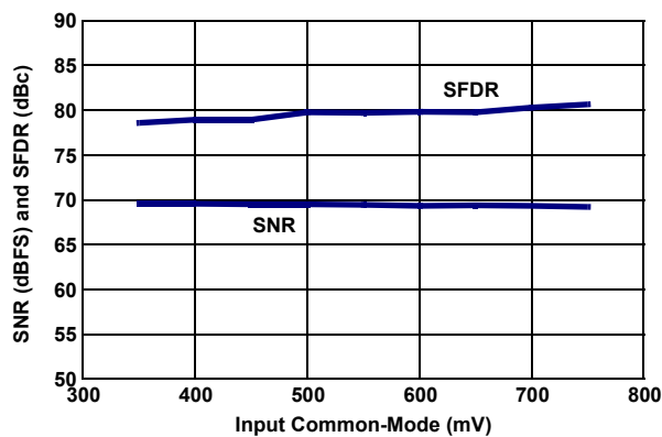
Figure 15. SNR and SFDR vs VCM
