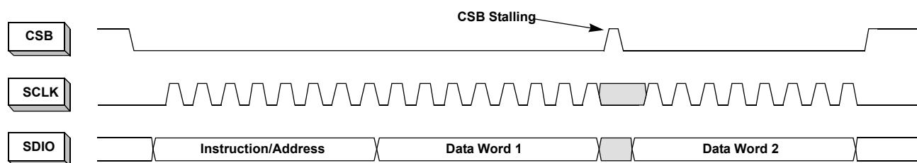
Figure 40. 2-Byte Transfer
