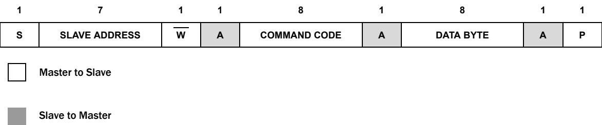
FIGURE 21. WRITE BYTE PROTOCOL
