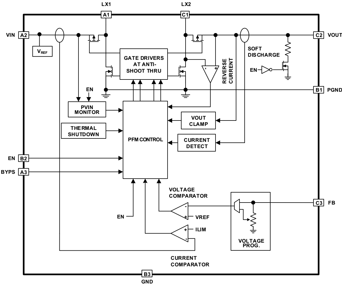
FIGURE 3. BLOCK DIAGRAM
