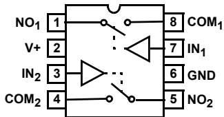
ISL84541 (SOT-23) TOP VIEW
