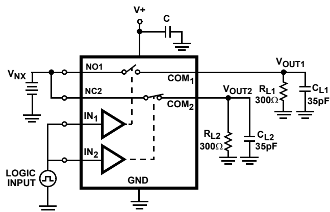
FIGURE 2. CHARGE INJECTION
