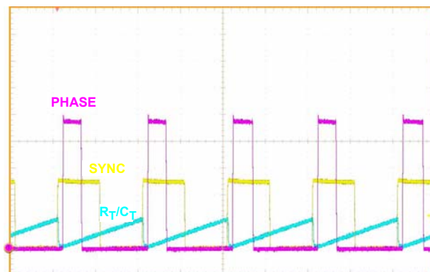
FIGURE 20. SYNCHRONIZATION OPERATION
