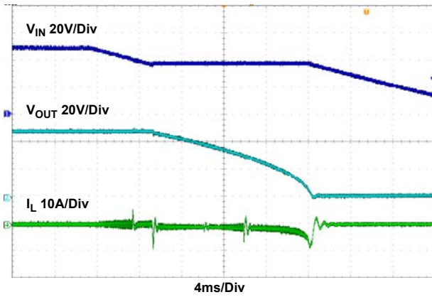
Figure 28. Bi-Direction Operation, V_{IN} = 48V , V_{in\_limit} = 36V , I_{IN} = 1A
