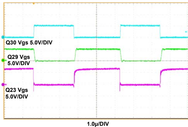
Figure 25. Gating Signals V_{IN} = 12V , I_{OUT} = 3A
