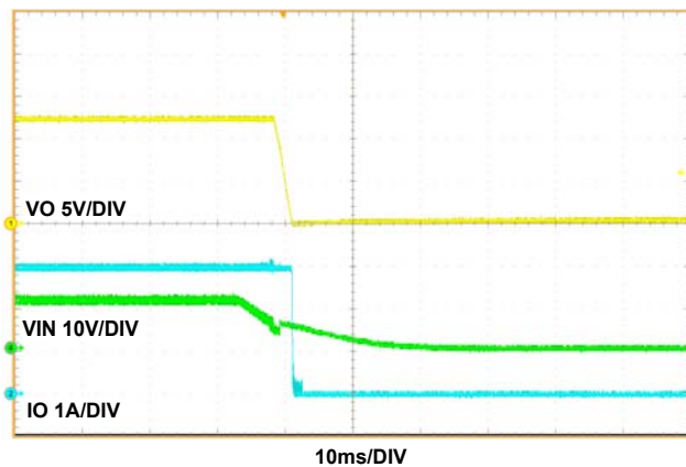
Figure 18. Shutdown Waveforms ( V_{IN} = 12V , I_{OUT} = 3A )
