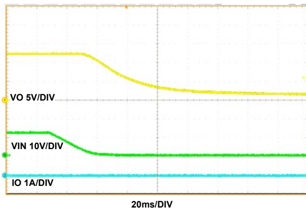
Figure 16. Shutdown Waveforms ( V_{IN} = 12V , I_{OUT} = 0A )
