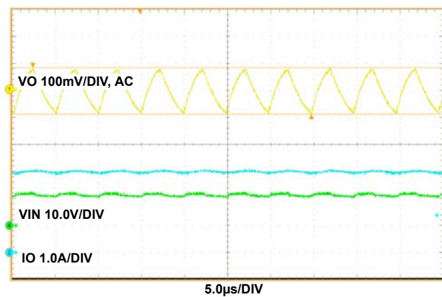
Figure 24. Output Ripple ( I_{OUT} = 3A , V_{IN} = 12V )
