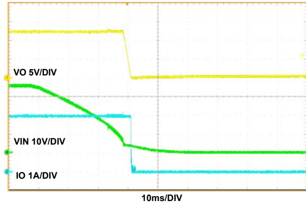
Figure 22. Shutdown Waveforms ( V_{IN} = 36V , I_{OUT} = 3A )
