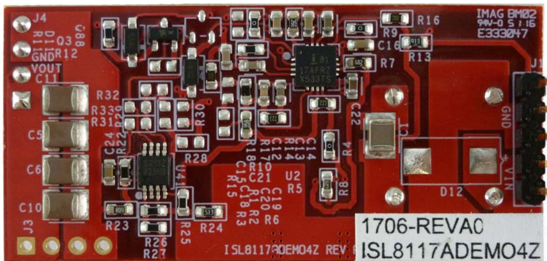
Figure 5. Bottom View
