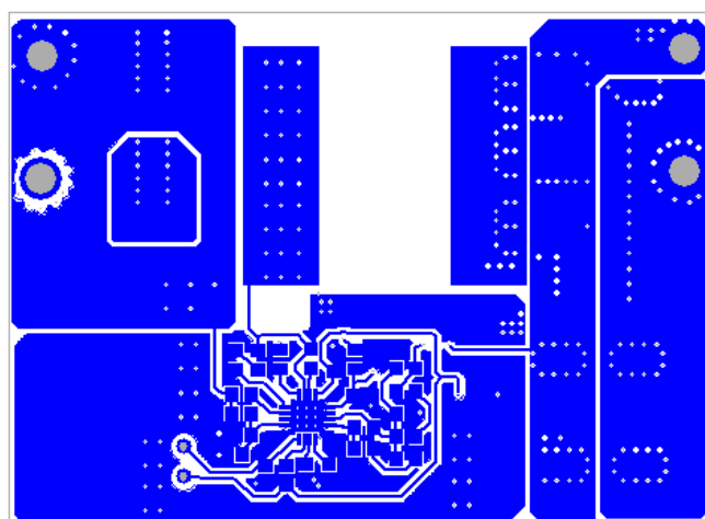
FIGURE 8. LAYER 1 - TOP
