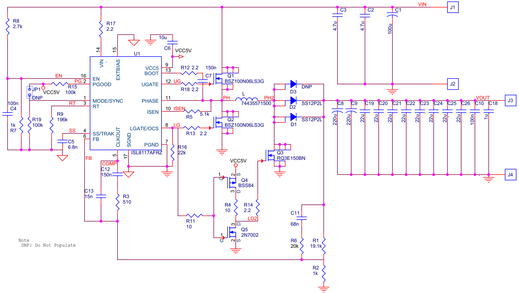
FIGURE 6. ISL8117A-LDEM02Z SCHEMATIC
