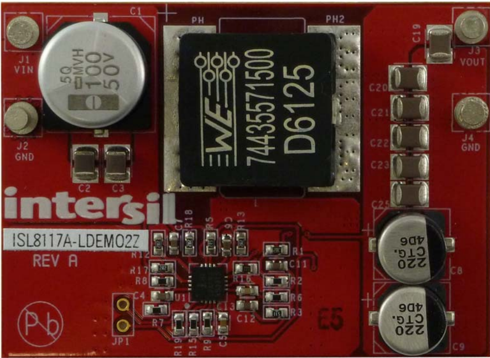
FIGURE 4. TOP VIEW
