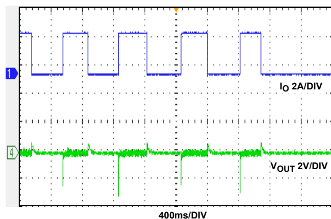
FIGURE 23. LOAD TRANSIENT, I_O = 0A TO 3A
