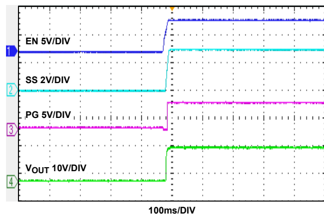
FIGURE 21. START-UP WAVEFORMS, I_O = 3A
