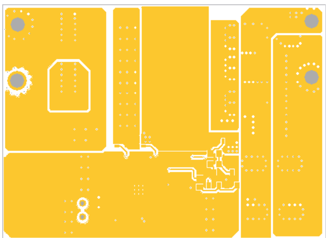
FIGURE 11. LAYER 4 - BOTTOM
