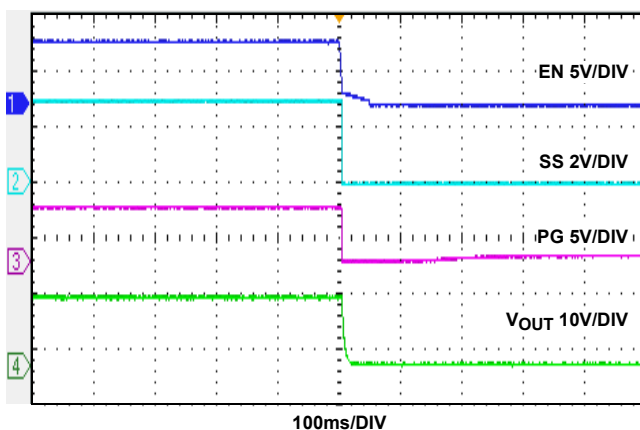
FIGURE 22. SHUT-DOWN WAVEFORMS, I_O = 3A
