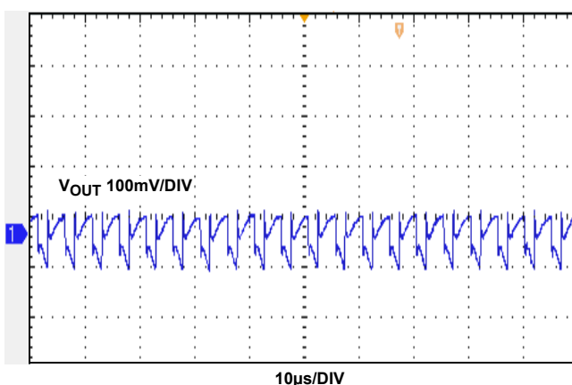
FIGURE 24. OUTPUT RIPPLE, I_O = 3A
