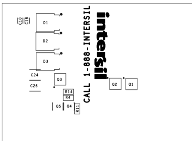
FIGURE 12. ASSEMBLY BOTTOM
