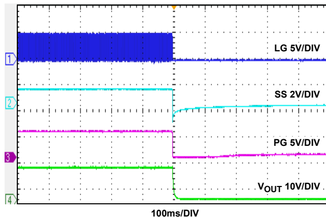
FIGURE 20. SHUT-DOWN WAVEFORMS, I_O = 3A
