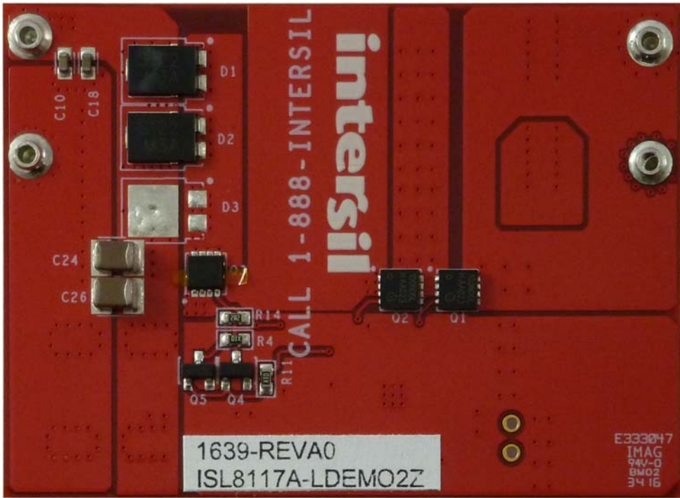
FIGURE 5. BOTTOM VIEW
