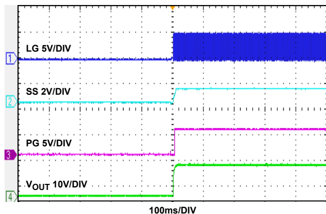
FIGURE 19. START-UP WAVEFORMS, I_O = 3A
