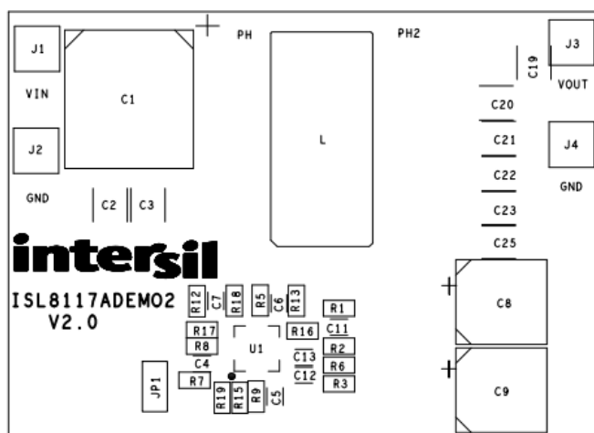
FIGURE 7. ASSEMBLY TOP
