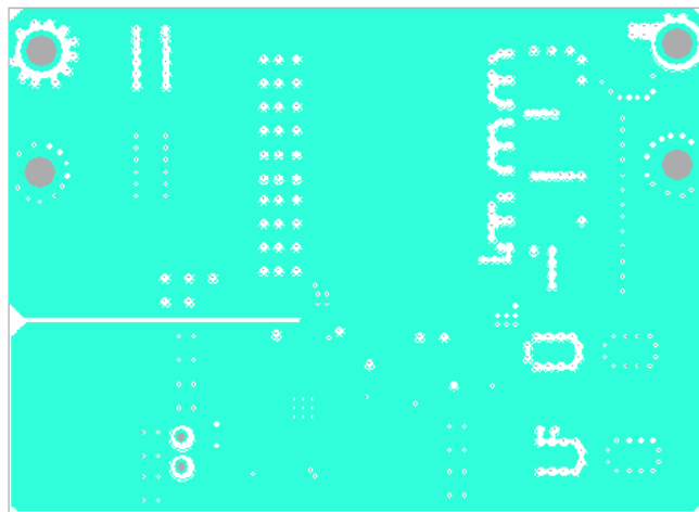
FIGURE 10. LAYER 3
