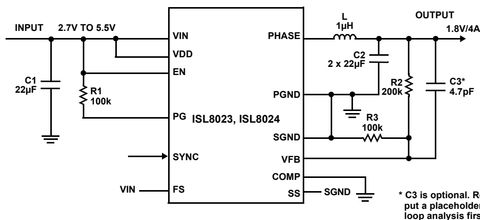
FIGURE 2. TYPICAL APPLICATION DIAGRAM
