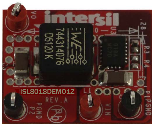
FIGURE 2. TOP SIDE
