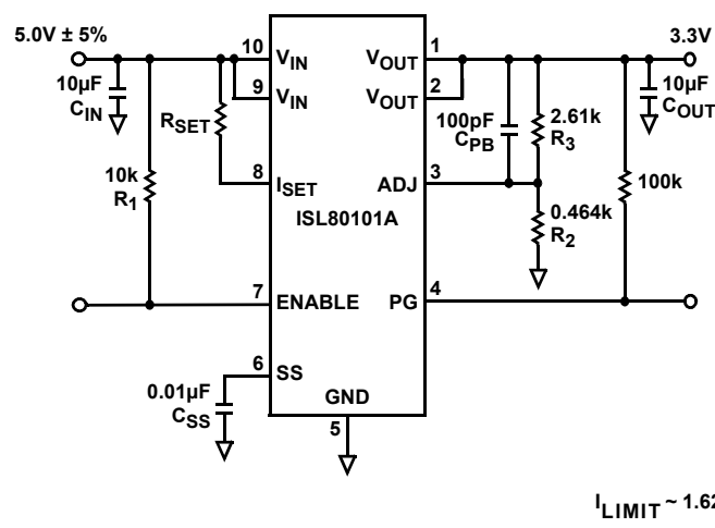
FIGURE 1. TYPICAL APPLICATION
