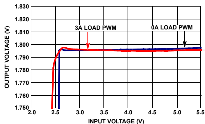
FIGURE 15. OUTPUT VOLTAGE REGULATION vs VIN (PWM V_{OUT} = 1.8 )
