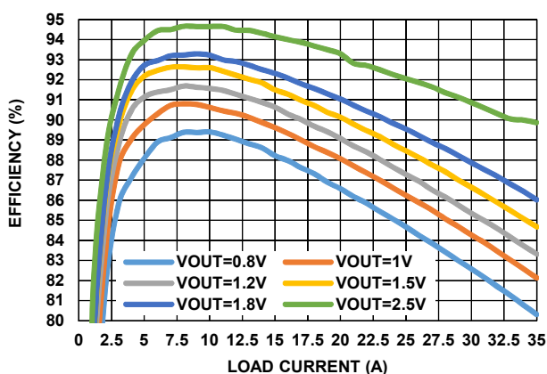
FIGURE 12. EFFICIENCY, V_{IN} = 5V , f_{SW} = 500kHz
