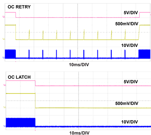
FIGURE 27. OVERCURRENT AND SHORT-CIRCUIT PROTECTION (CH1-VOUT, CH2-PGOOD, CH3-PHASE)
