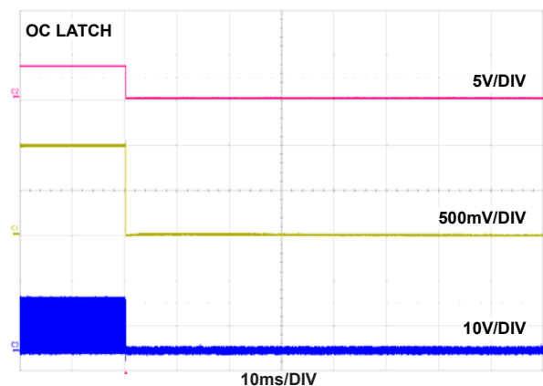
FIGURE 29. OVERCURRENT AND SHORT-CIRCUIT PROTECTION (CH1-VOUT, CH2-PGOOD, CH3-PHASE)
