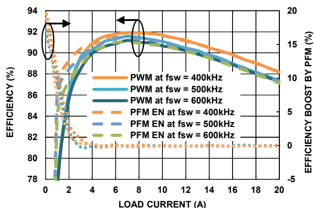
FIGURE 16. EFFICIENCY COMPARISON OF PWM AND PFM ENABLED MODE, V_{IN} = 5V , V_{OUT} = 1V
