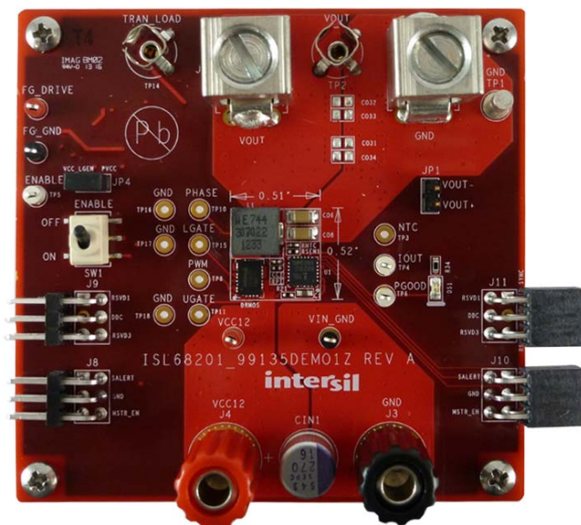
FIGURE 2. DEMONSTRATION BOARD TOP VIEW
