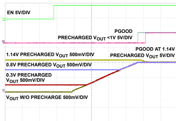
FIGURE 18. POWER-UP WITH/WITHOUT PRECHARGED LOAD
