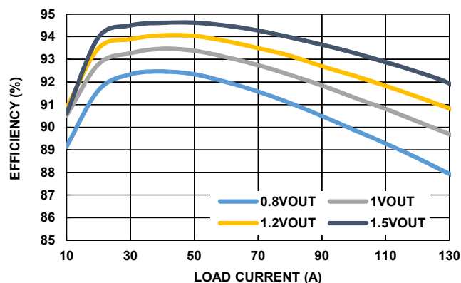
FIGURE 10. 3-PHASE EFFICIENCY
