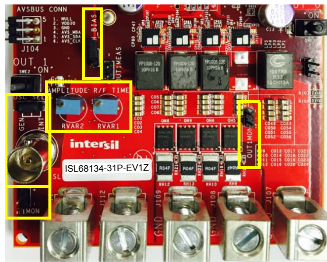
FIGURE 4. MEASUREMENT POINTS
