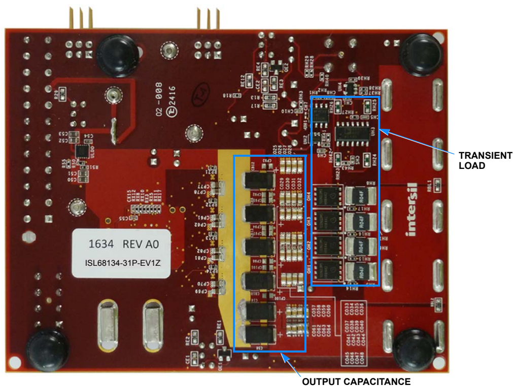
FIGURE 9. BOTTOM SIDE
