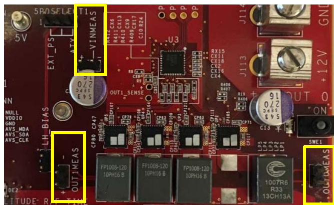
FIGURE 3. TEST POINTS
