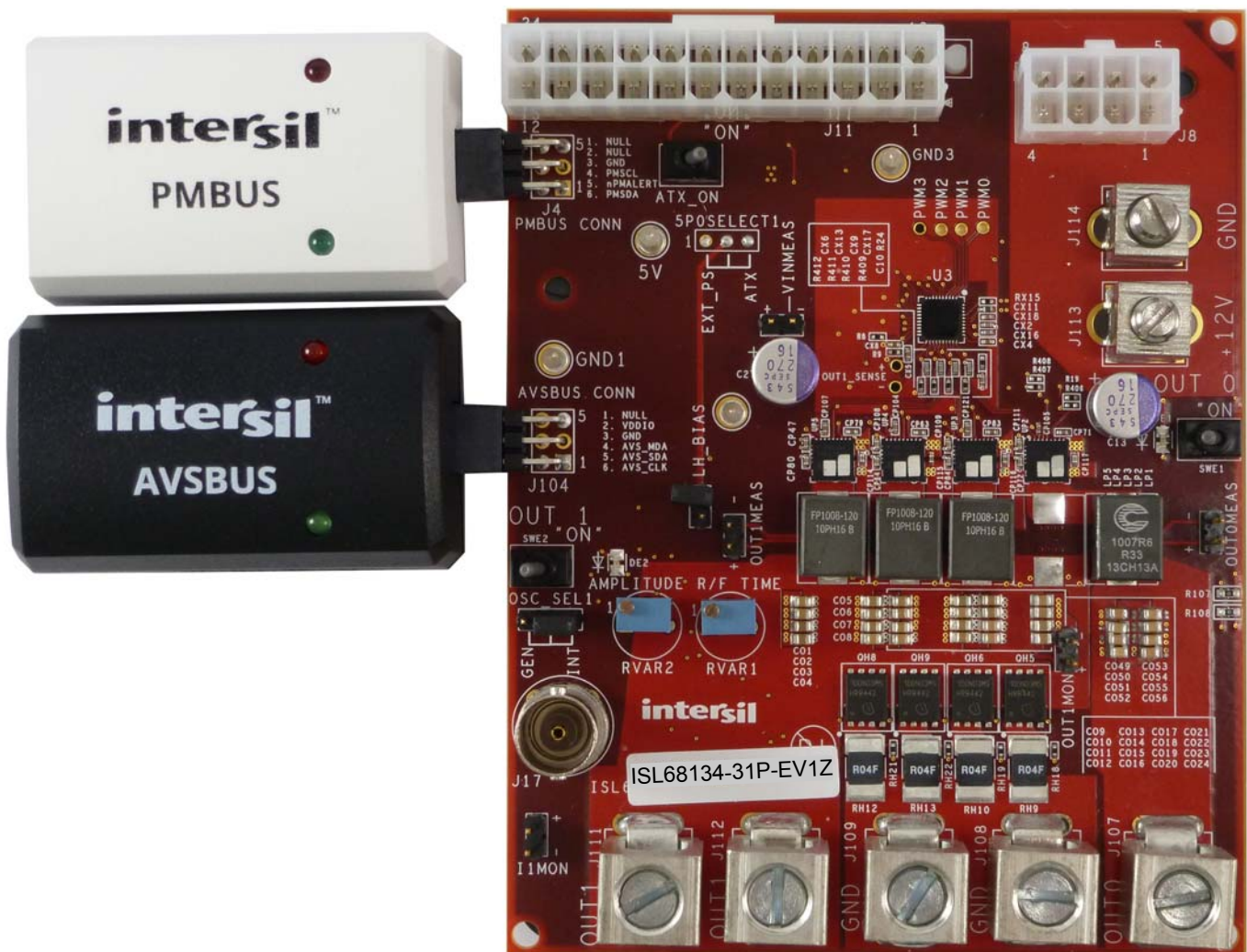
FIGURE 2. CONNECTIONS
