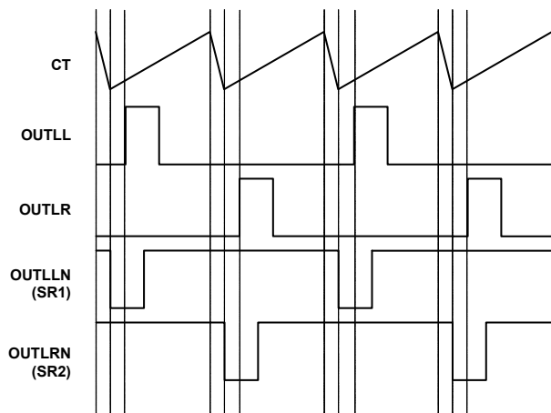
FIGURE 24. WAVEFORM TIMING WITH PWM OUTPUTS DELAYED, 0\text{V} < V_{\text{ADJ}} < 2.425\text{V}
