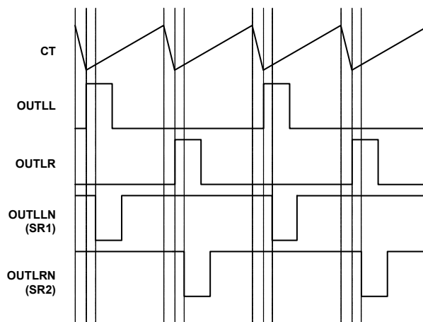
FIGURE 25. WAVEFORM TIMING WITH SR OUTPUTS DELAYED, 2.575\text{V} < V_{\text{ADJ}} < 5.00\text{V}
