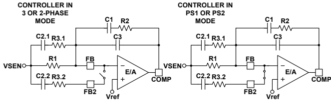
FIGURE 15. FB2 FUNCTION IN 2-PHASE MODE
