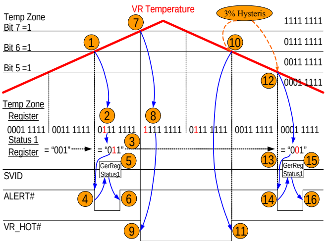
FIGURE 14. VR_HOT#/ALERT# BEHAVIOR
