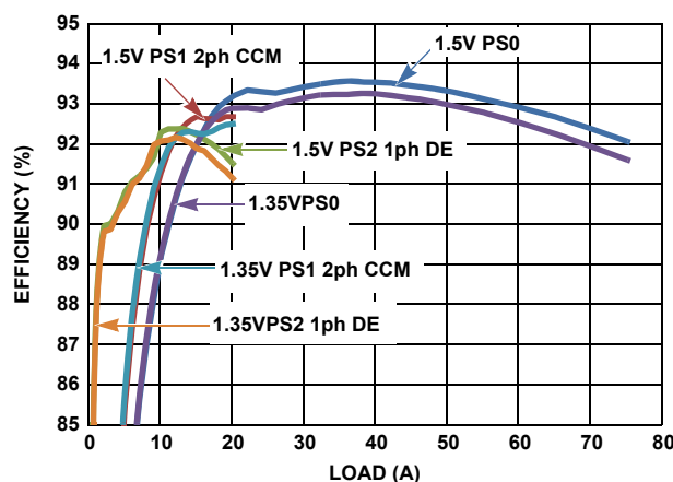
FIGURE 2. ISL6353EVAL1Z EFFICIENCY vs LOAD
