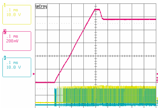
FIGURE 36. 2-PHASE CPU MODE SOFT-START, VIN = 19V, I0 = 0A, VID = 0.95V, Ch1: PHASE1, Ch2: VOUT, Ch3: PHASE2
