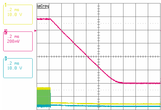
FIGURE 37. 2-PHASE CPU MODESHUT DOWN, VIN = 19V, I0 = 1A, VID = 0.95V, Ch1: PHASE1, Ch2: VOUT, Ch3: PHASE2
