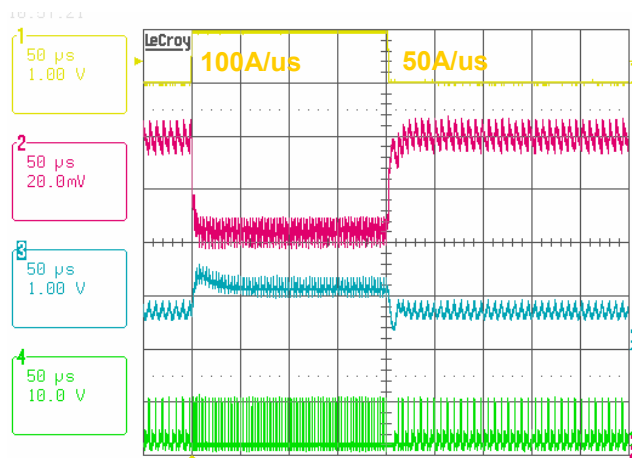
FIGURE 36. LOAD TRANSIENT RESPONSE IN ENHANCED DEM, V_{IN} = 8V , I_O = 2A \leftrightarrow 20A , VID = 1.1V, Ch1: Io, Ch2: Vo, Ch3: Vcomp, Ch4: PHASE
