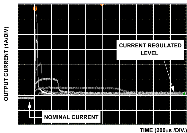
FIGURE 7. OC TO CR SETTLING TIME WAVEFORMS
