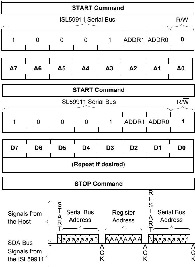
FIGURE 18. CONFIGURATION REGISTER READ
