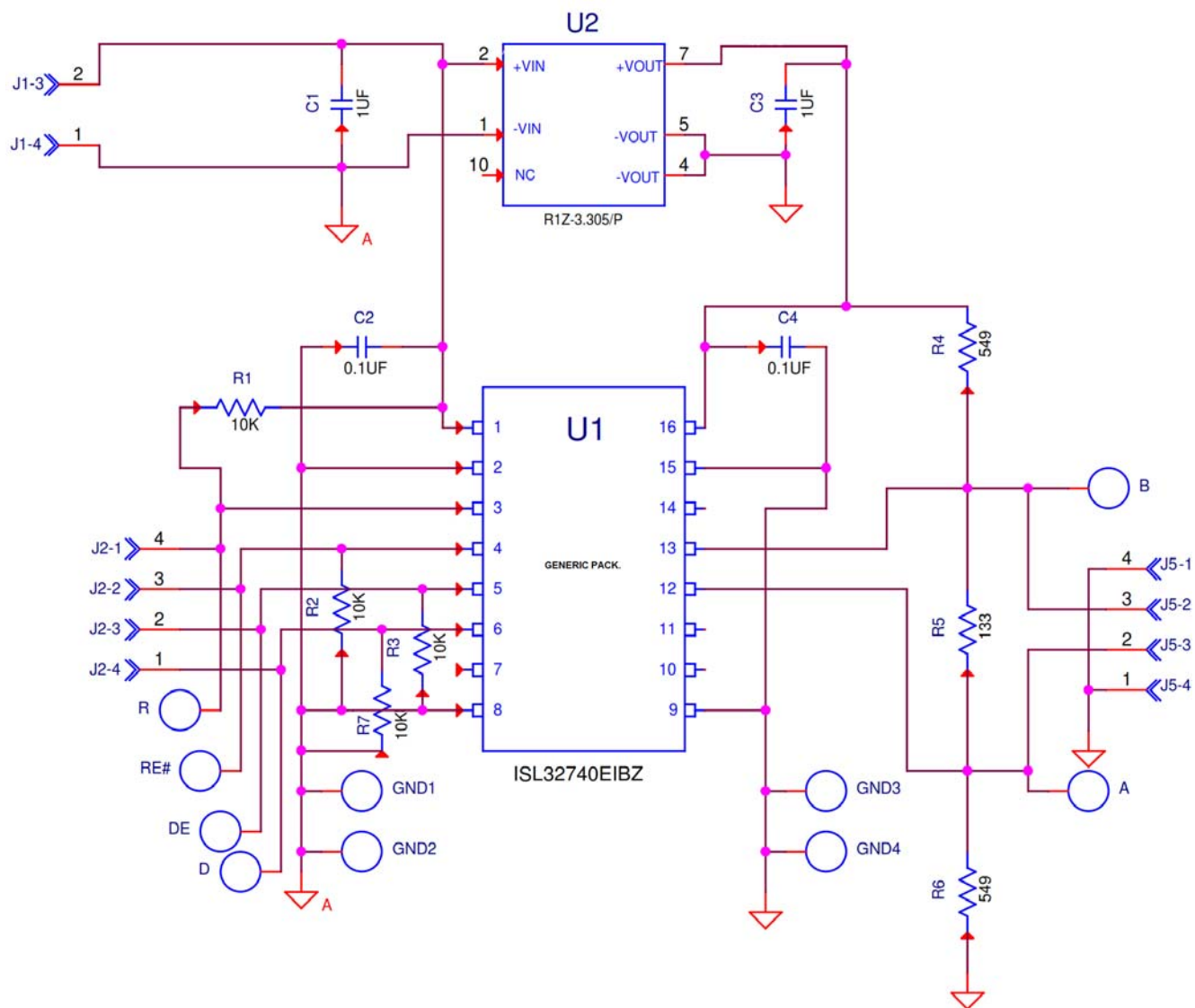
Figure 4. ISL32740EVAL1Z Schematic
