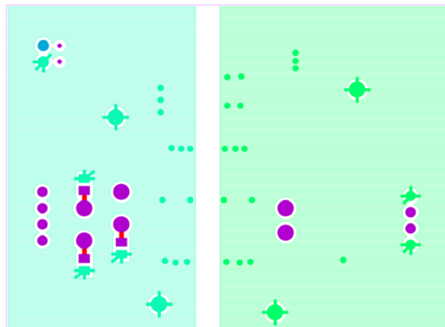
Figure 8. Bottom Layer
