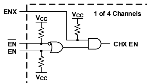
FIGURE 33. ISL32x77E ENABLE LOGIC
