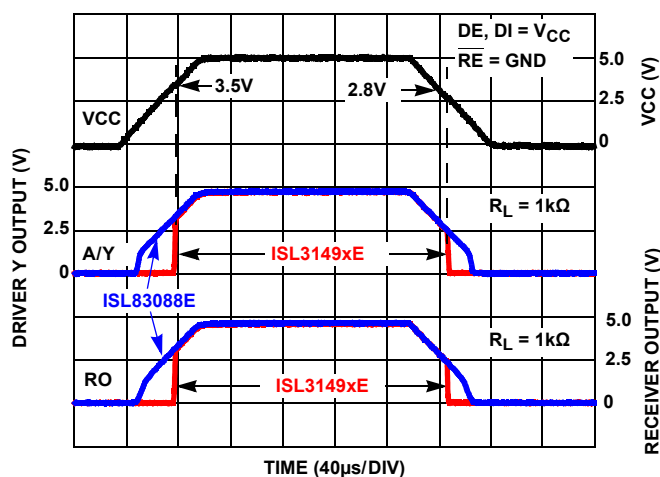
FIGURE 12. HOT PLUG PERFORMANCE (ISL3149xE) vs ISL83088E WITHOUT HOT PLUG CIRCUITRY
