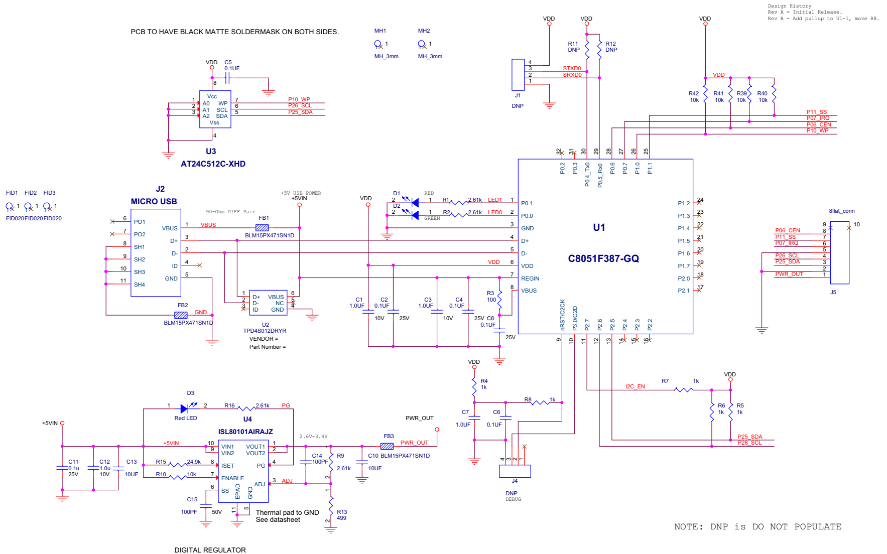
FIGURE 5. ISLI2UEV1Z SCHEMATIC
