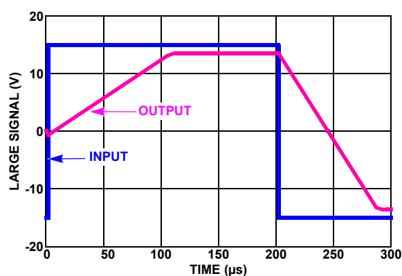
FIGURE 65. SIMULATED LARGE SIGNAL 10V STEP RESPONSE
