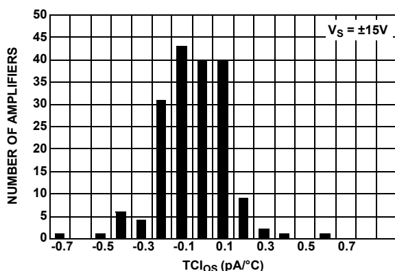
FIGURE 19. TC_{los} vs NUMBER OF AMPLIFIERS, V_S = \pm 15V
