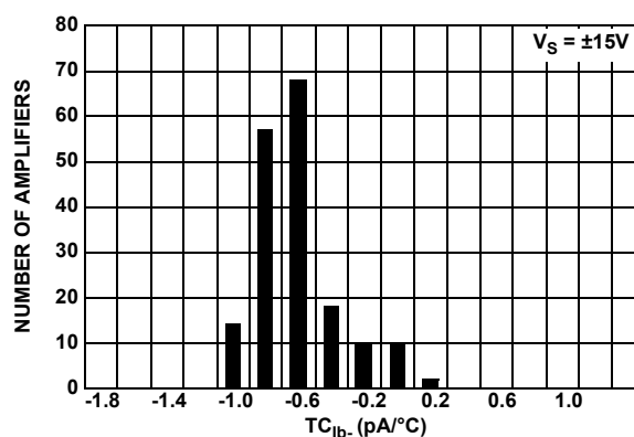
FIGURE 16. TC_{ibo} vs NUMBER OF AMPLIFIERS, V_S = \pm 15V
