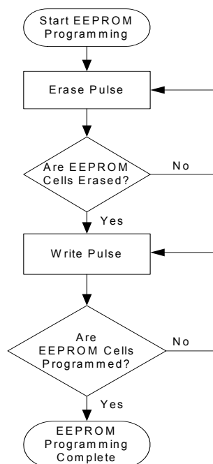
FIGURE 12. EEPROM PROGRAMMING FLOWCHART
