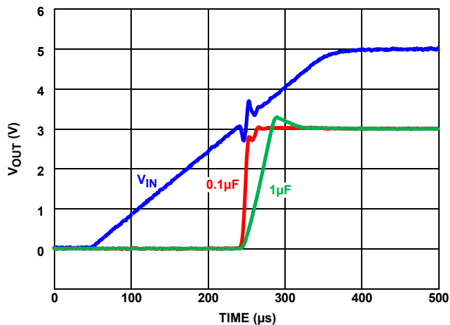
FIGURE 97. TURN-ON TIME
