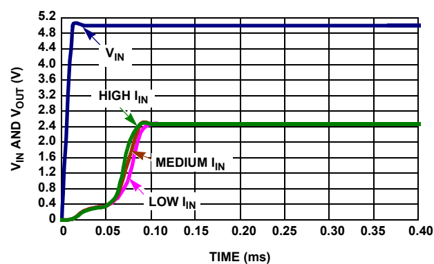
FIGURE 25. TURN-ON TIME
