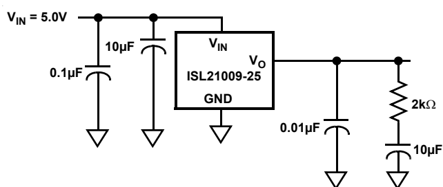
FIGURE 58. HANDLING HIGH LOAD CAPACITANCE
