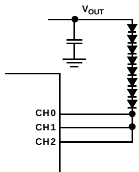
FIGURE 38. GROUPING MULTIPLE CHANNELS FOR HIGH CURRENT APPLICATIONS
