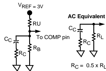
FIGURE 9. COMPENSATION CIRCUIT
