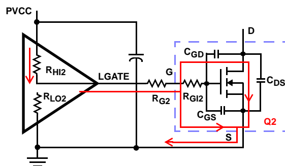
FIGURE 19. TYPICAL LOWER-GATE DRIVE TURN-ON PATH
