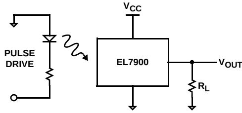
FIGURE 1. RISE/FALL TIME MEASUREMENT Typical Performance Curves
