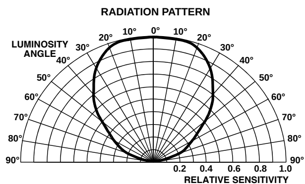
FIGURE 8. RADIATION PATTERN
