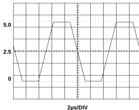
FIGURE 24. OUTPUT SWING
