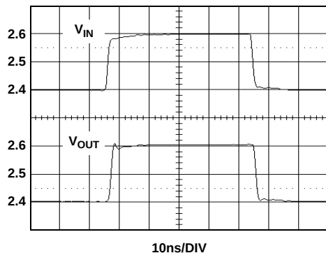
FIGURE 23. SMALL SIGNAL TRANSIENT REPNSE
