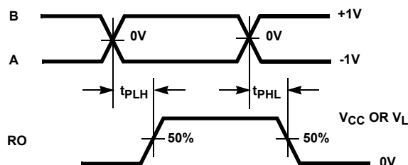
FIGURE 1B. MEASUREMENT POINTS
