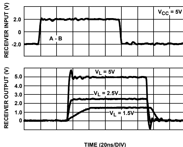
FIGURE 15. RECEIVER WAVEFORMS
