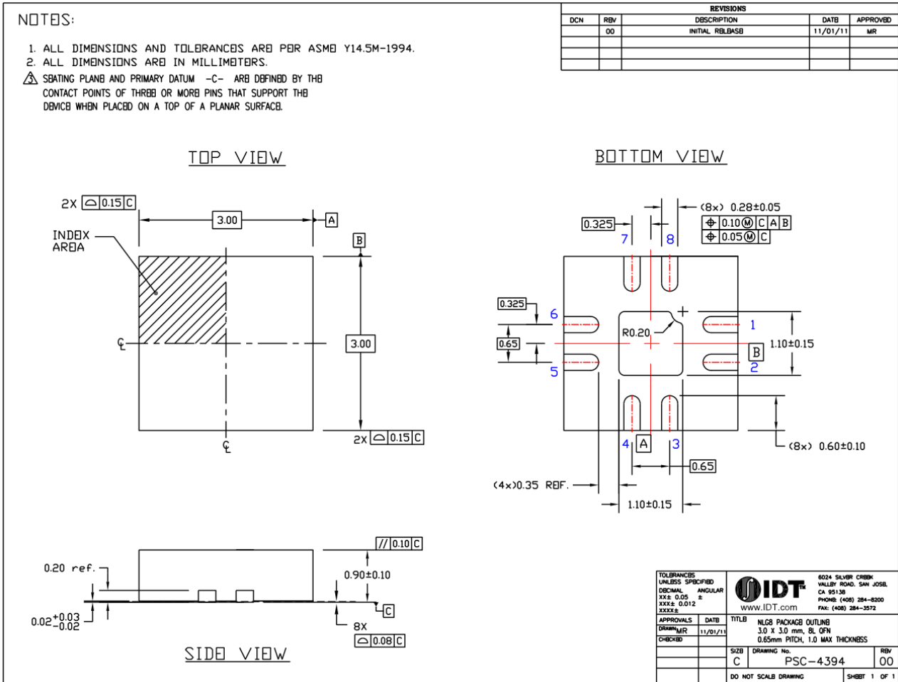
Figure 8. Package Outline Drawing (NLG8 QFN-8 3.0mmx3.0mmx1mm 8-ld, 0.65mm pitch)
