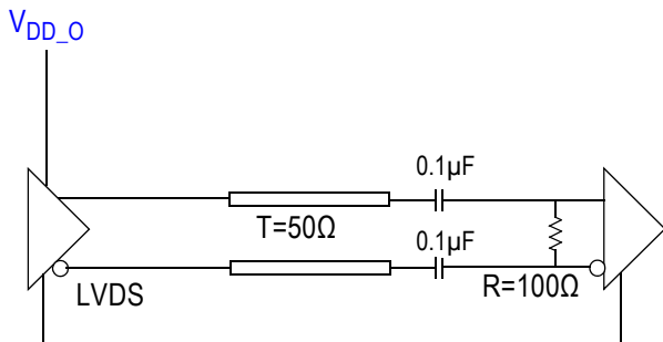
Figure 9. LVDS (STYLE = 0) AC Coupling
