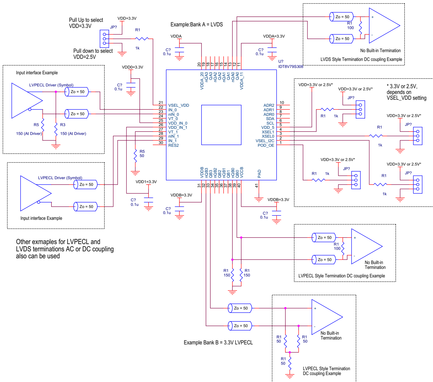
Figure 6. Application Information
