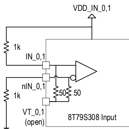
Figure 16. Unused Input
