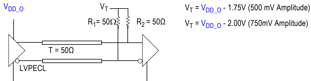
Figure 10. Output Termination
