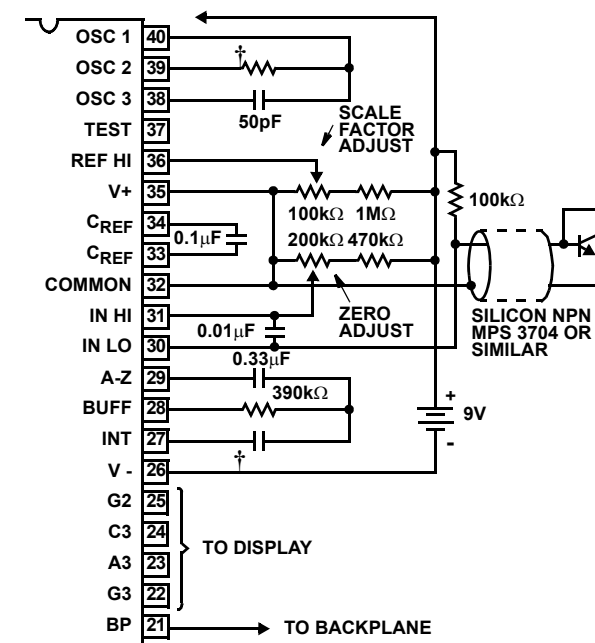
FIGURE 15. ICL7126 MEASURING RATIOMETRIC VALUES OF QUAD LOAD CELL
