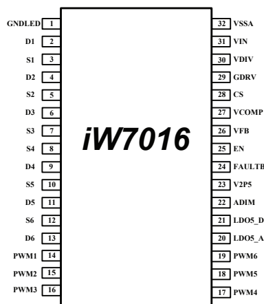
Figure 4.1 : SOP-32
