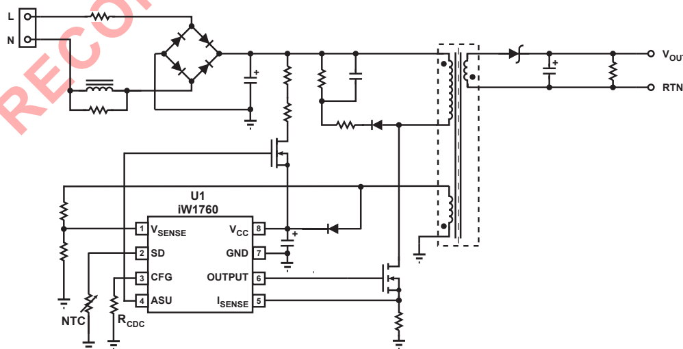
Figure 3.1: iW1760 Typical Application Circuit (Using Depletion Mode N-FET as Active Start-up Device)
