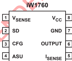
Figure 4.1: 8 Lead SO-8 Package
