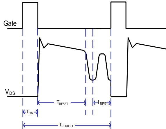
Figure 10.2 : V DS Timing
