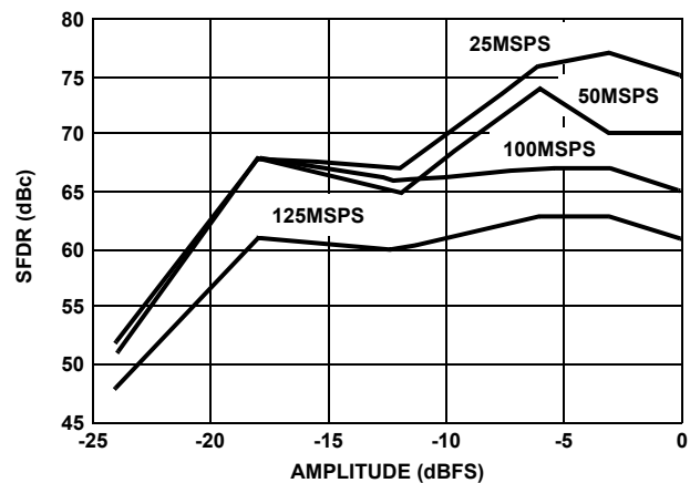
FIGURE 6. SFDR vs AMPLITUDE, f_{CLK}/f_{OUT} = 10
