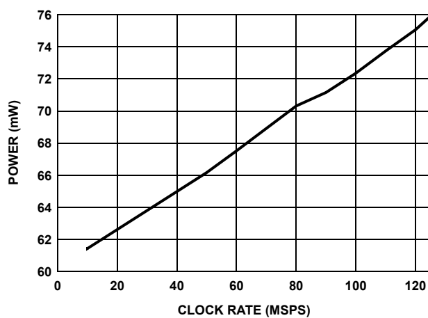
FIGURE 38. POWER vs CLOCK RATE, f_{CLK}/f_{OUT} = 10 , I_{OUT} = 20\text{mA}
