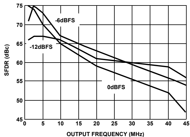
FIGURE 4. SFDR vs f_{OUT} , CLOCK = 100MSPS
