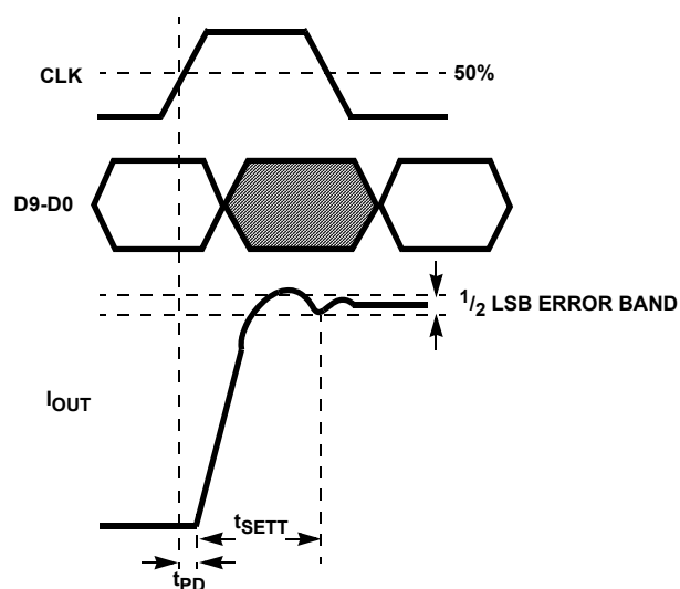
FIGURE 39. OUTPUT SETTLING TIME DIAGRAM
