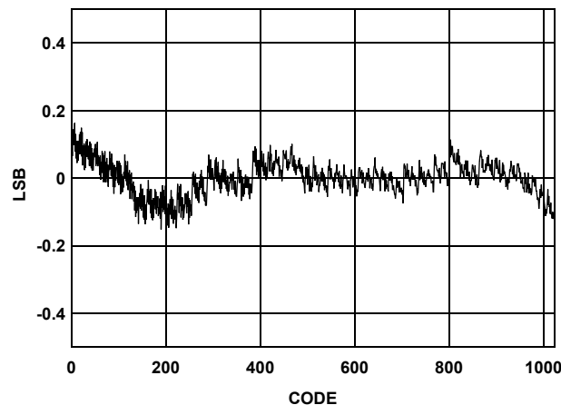
FIGURE 18. INTEGRAL NONLINEARITY
