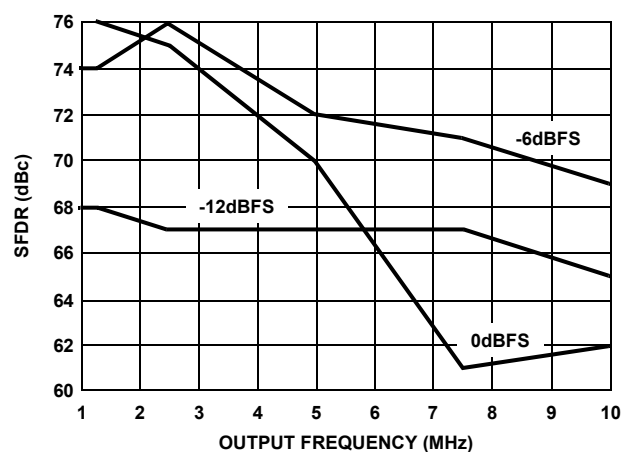
FIGURE 2. SFDR vs f_{OUT} , CLOCK = 25MSPS
