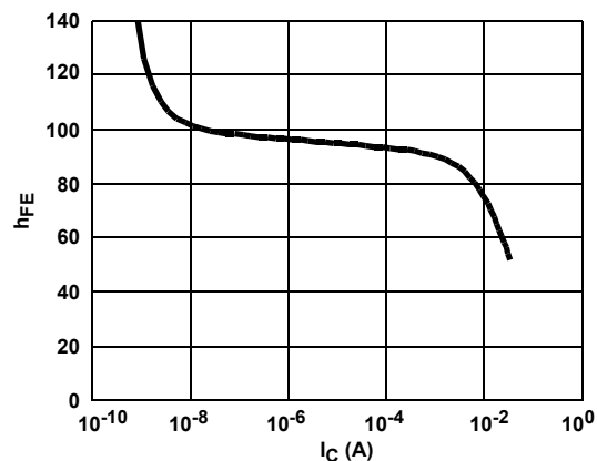
FIGURE 2. h_{FE} vs I_C
