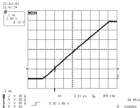
FIGURE 19. OUTPUT SOFT-START
