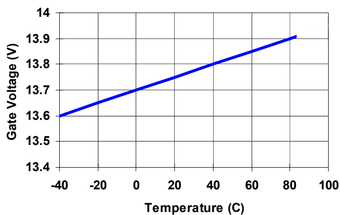
FIGURE 14. GATE VOLTAGE VS TEMPERATURE, V_{DD} = 80V
