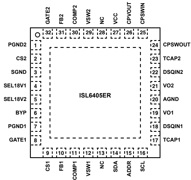
ISL6405 (QFN) TOP VIEW
