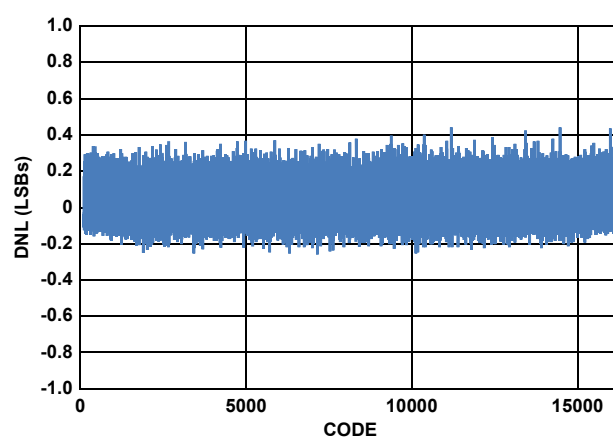
FIGURE 10. DIFFERENTIAL NONLINEARITY
