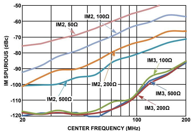
FIGURE 13. IM2 AND IM3 vs R_{LOAD}
