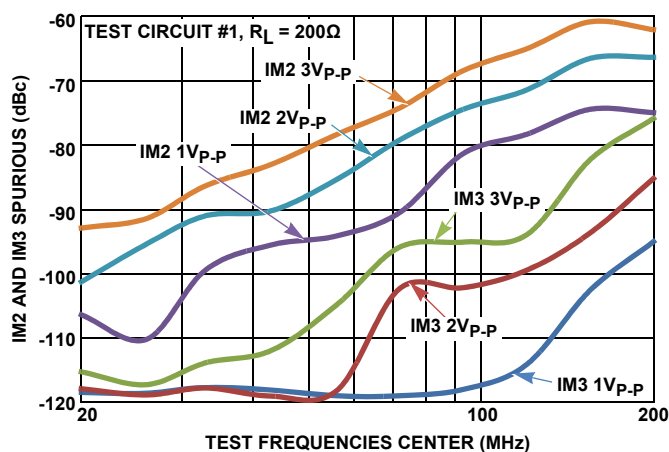
FIGURE 9. IM2 AND IM3 vs OUTPUT SWING
