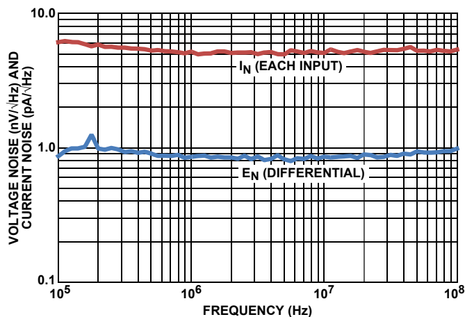
FIGURE 15. INPUT VOLTAGE AND CURRENT SPOT NOISE
