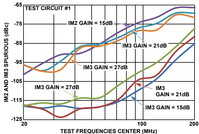
FIGURE 11. IM2 AND IM3 vs GAIN
