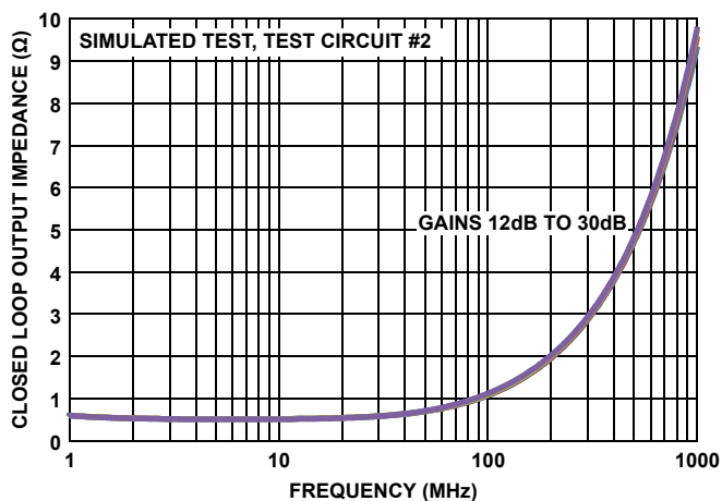
FIGURE 17. DIFFERENTIAL OUTPUT IMPEDANCE
